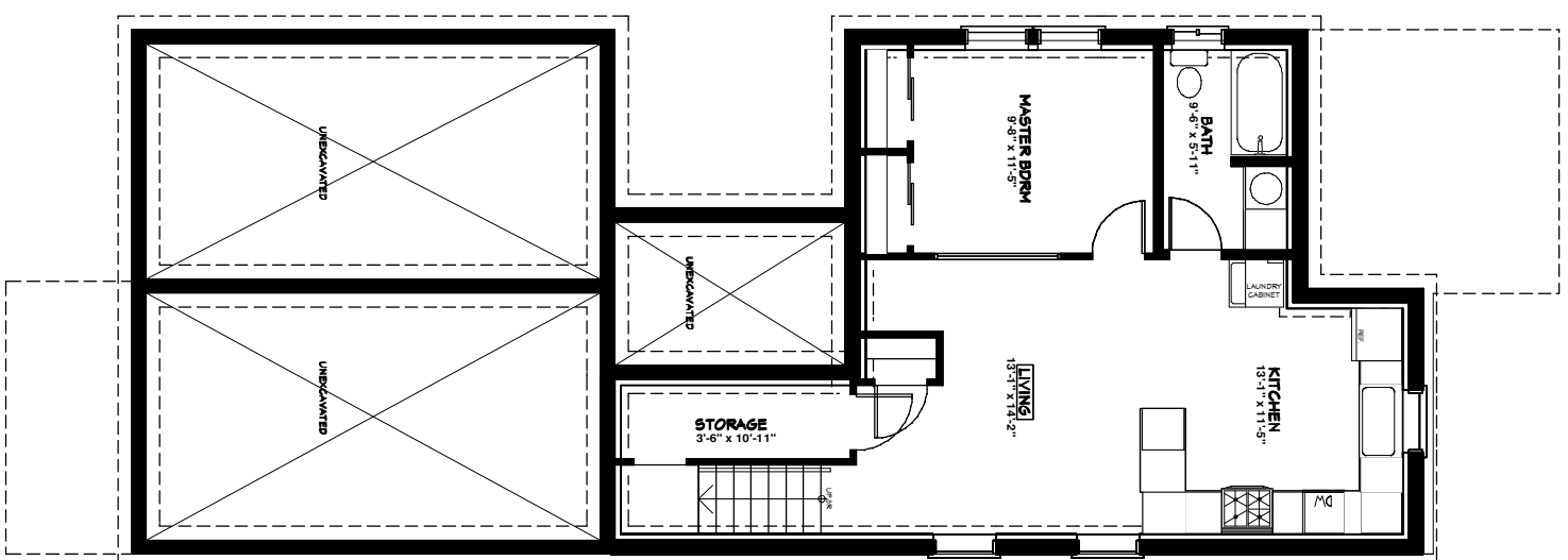
○ BASEMENT FLOOR PLAN
